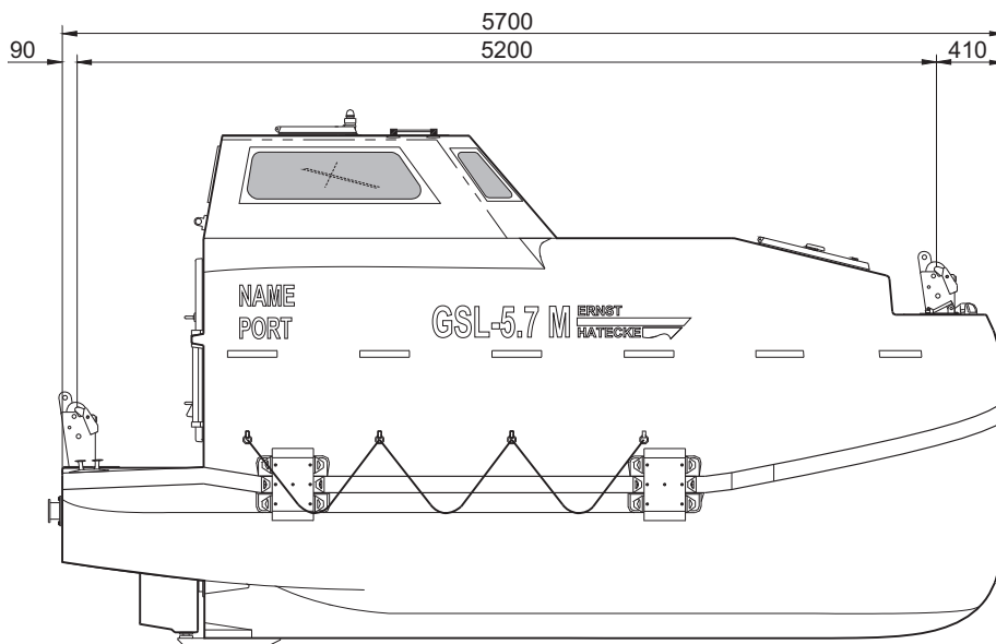
Scale 1:50
